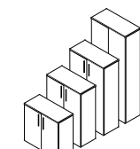
Шкаф 800x400x750 800x400x1100 800x400x1450 800x400x1800 800x400x2000
